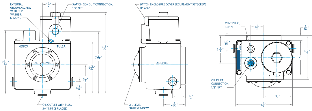
Model KLCP Oil Level Controller with Pneumatic Oil Level Switch
