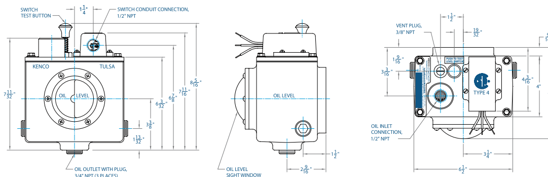
Model KLCM Oil Level Controller with Electric Switch in CSA® Type 4 Enclosure
