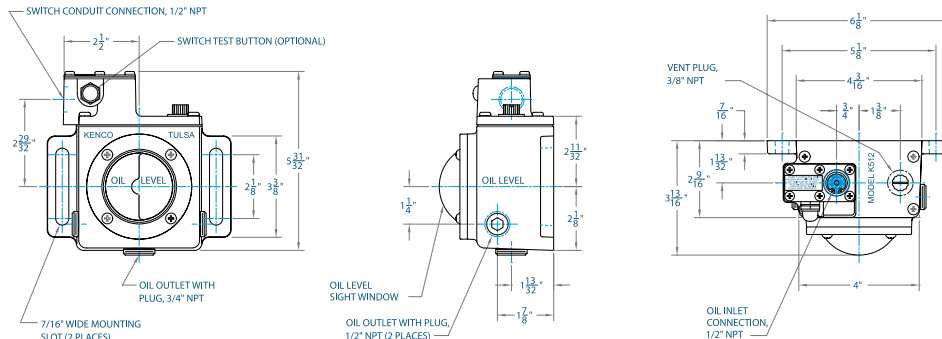
Model KLCE / *KES / KHL / *KHL-ES / KSHL / *KSHL-ES / KSLL / *KSLL-ES Oil Level Controllers with Switch in Explosion Proof Enclosure *Models KES / KHL-ES / KSHL-ES / KSLL-ES are Electric Oil Level Switches Only and have No Oil Inlet Connection and No Oil Level Controller Function
