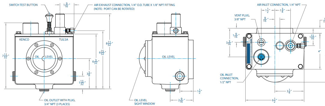
Model KLCM Oil Level Controller with Electric Switch in CSA® Type 4 Enclosure
