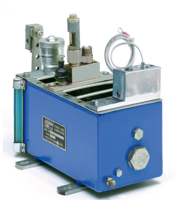
MODEL K507L SHOWN MOUNTED
