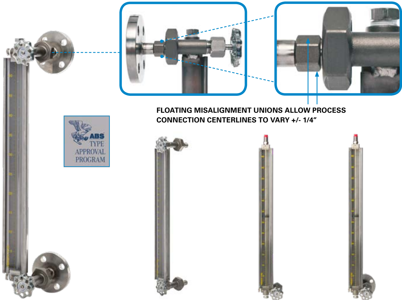
K9900 Bulk Tank Gauge w/ Threaded Connections
