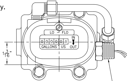
1/2" MNPT SWITCH CONDUIT CONNECTION (MODEL 14308 ONLY)
