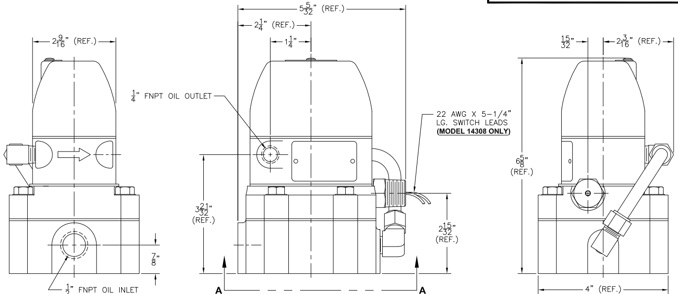
1/2" MNPT SWITCH CONDUIT CONNECTION (MODEL 14308 ONLY)
